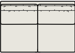
5XALP POWER RECLINE ARMLESS LOVESEAT 60w 23d 36h Inside: 23d 19h
